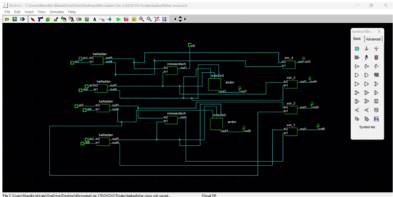
Fig 1 :CMOS Ladner Fischer Prefix Adder
